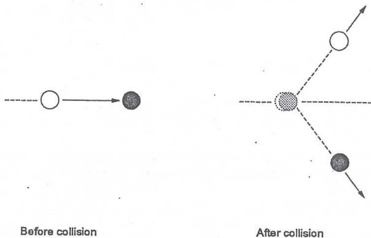
Figure 8. Elastic Scattering
