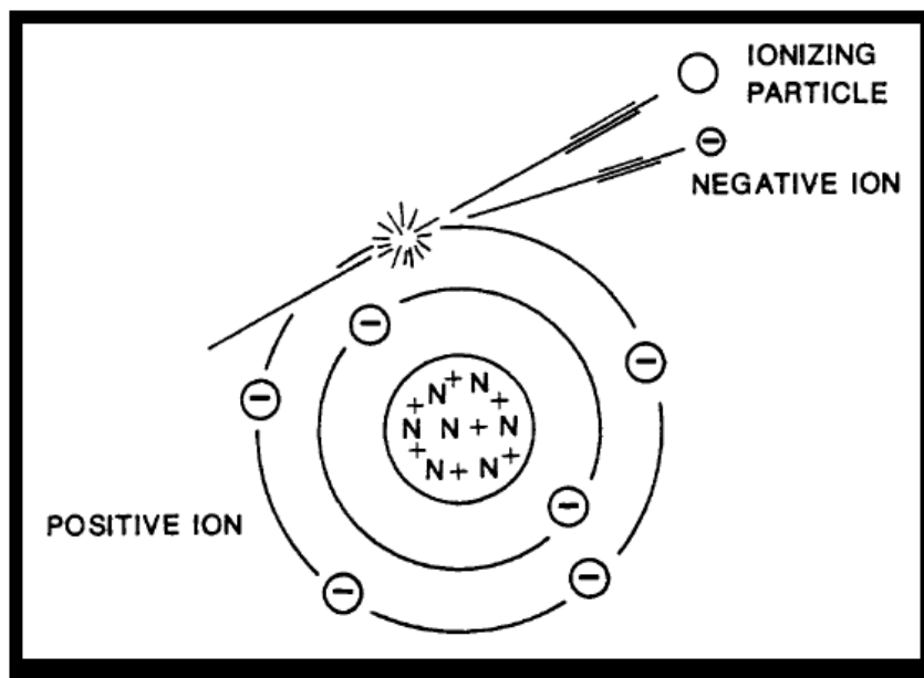
Figure 1. Ionization
