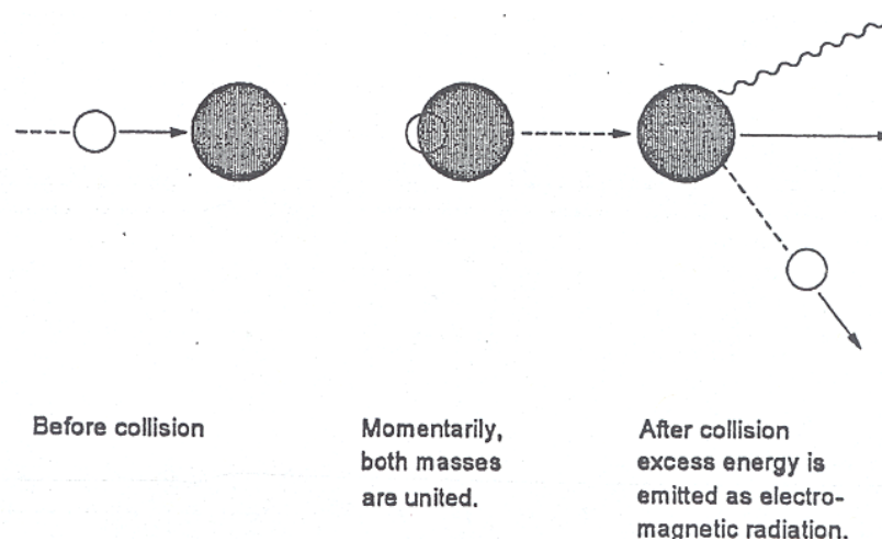
Figure 9. Inelastic Scattering
