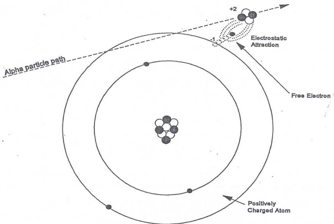
Figure 3. Ionization by an Alpha Particle
