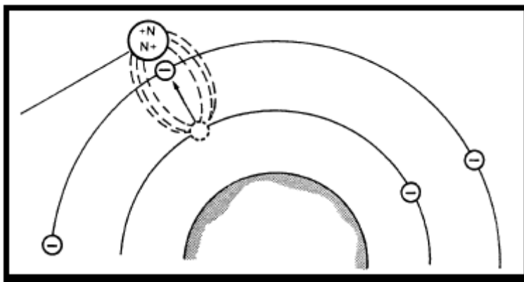
Figure 2. Electron Excitation
