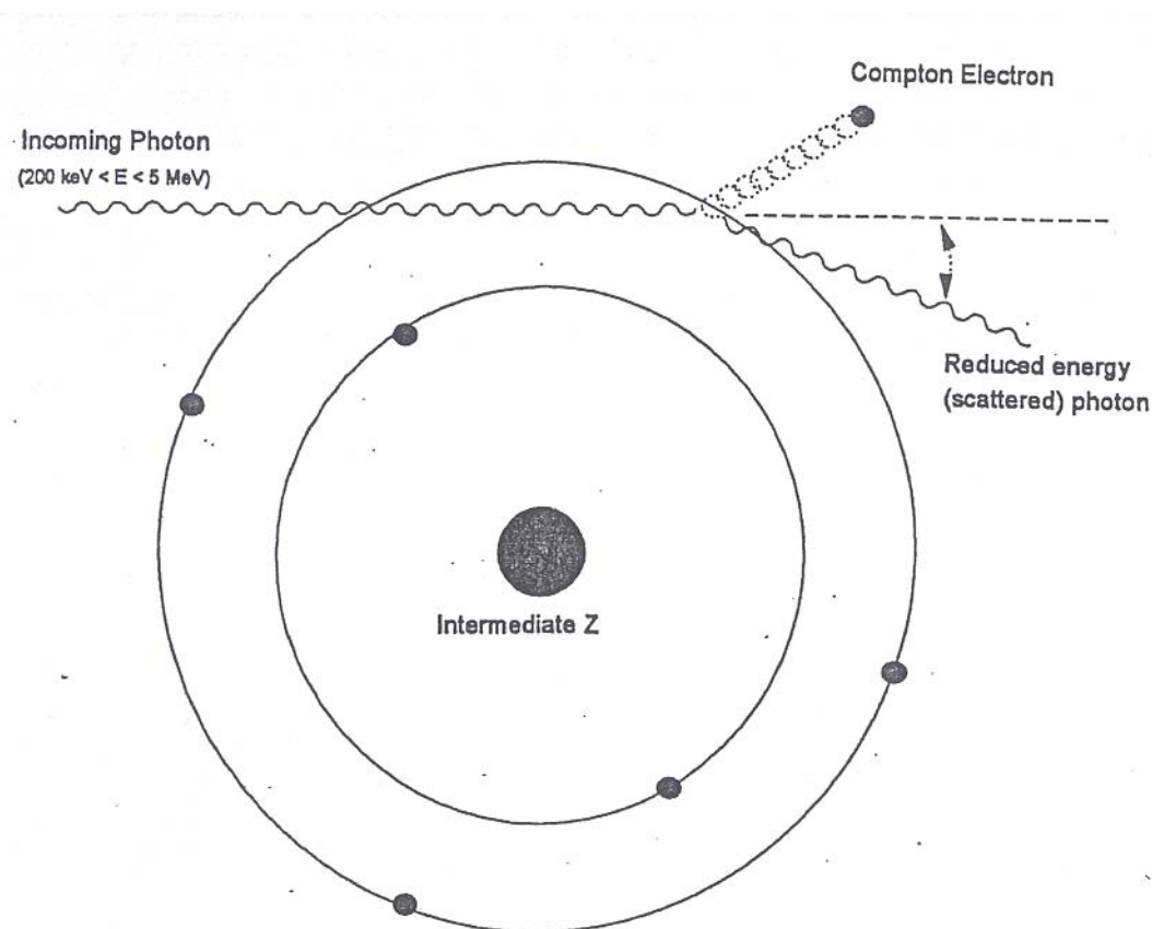
Figure 6. Compton Scattering
