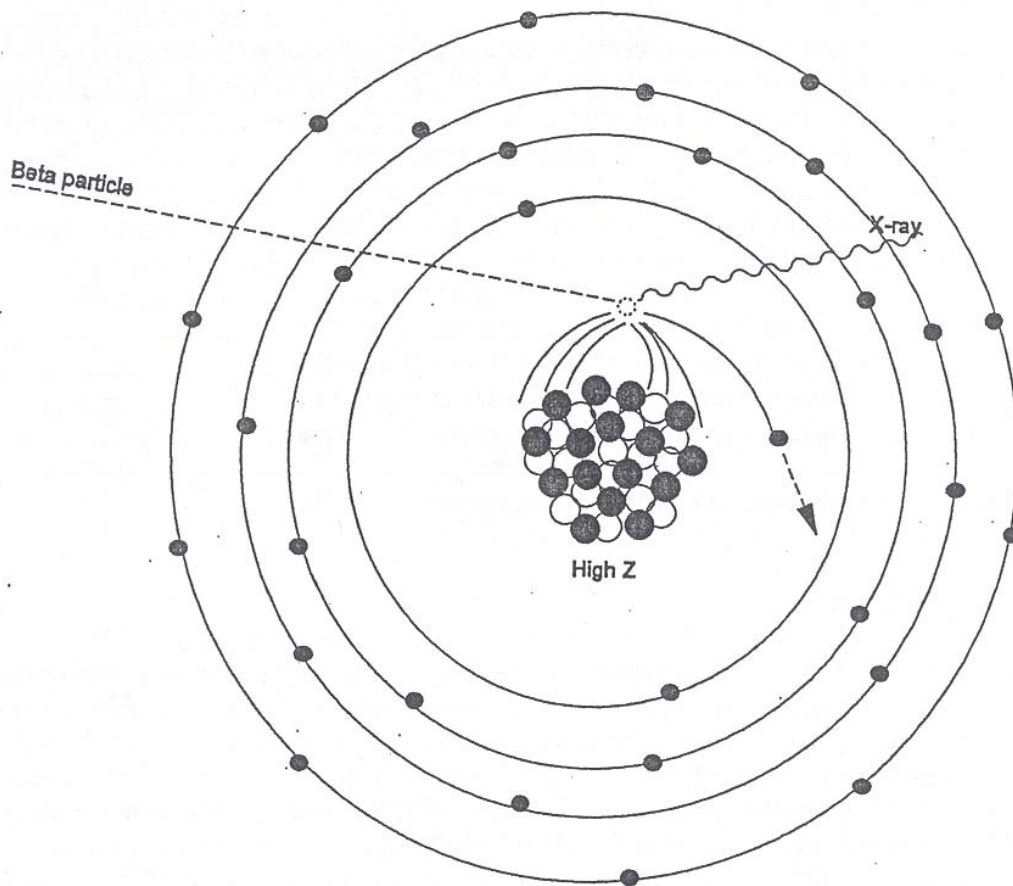
Figure 4. Bremsstrahlung Radiation
