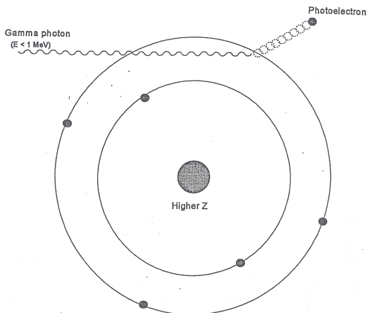
Figure 5. Photoelectric Effect
